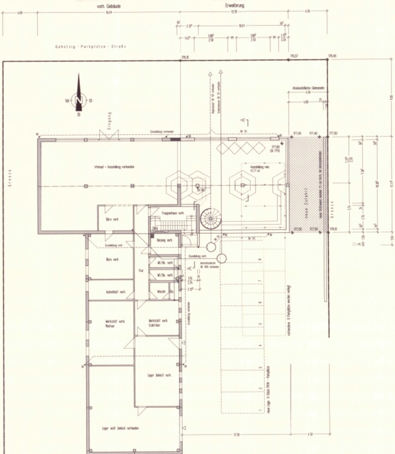
Grundriß Erdgeschoß
